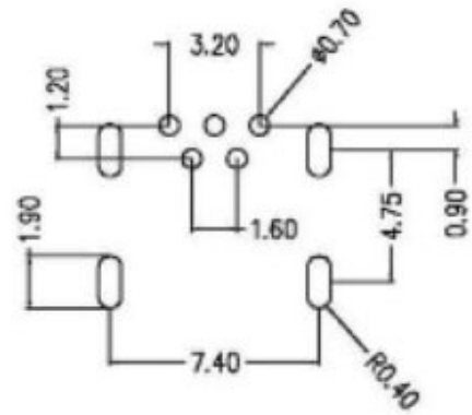
PCB LAYOUT
